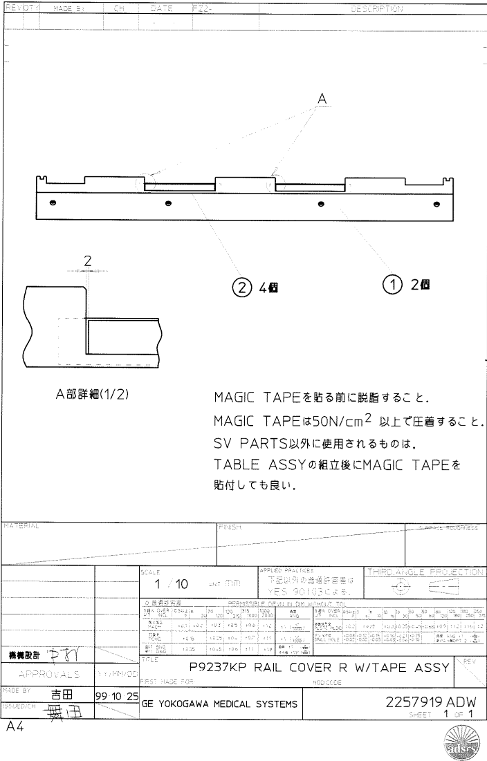
Figure 2-17 Rail Cover R W/Tape Assy (2257919ADW, Rev 0)
