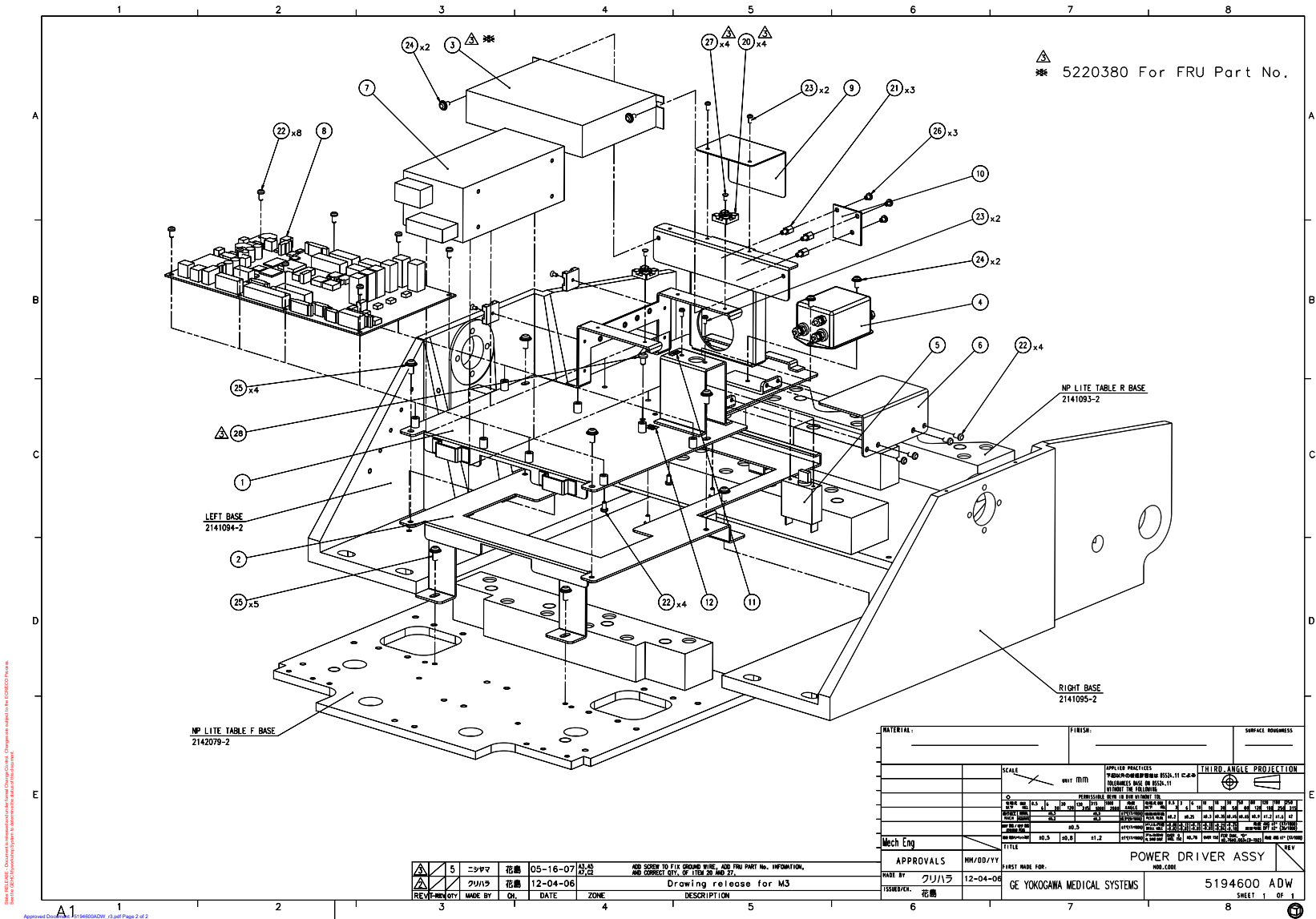
Figure 2-18 Power Driver Assy Positioning BSD Lite (5194600ADW, Rev 3)
