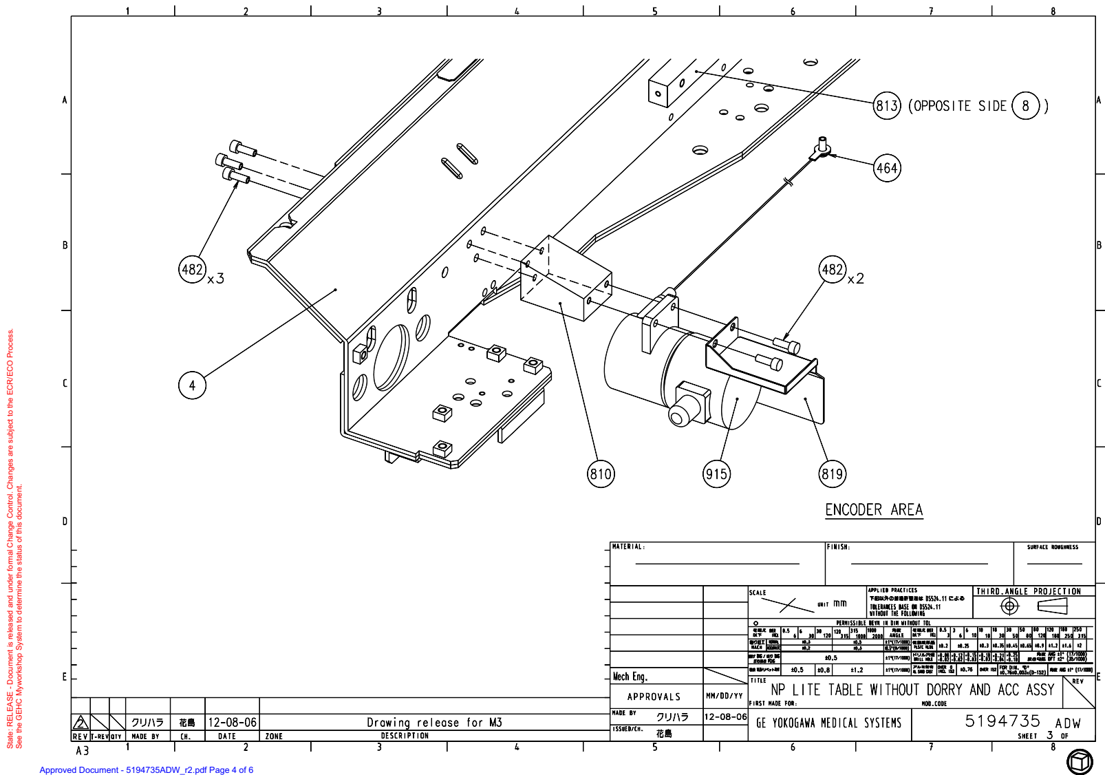
Figure 2-11 NP Lite Table (5194735ADW Sheet 3, Rev 2)
