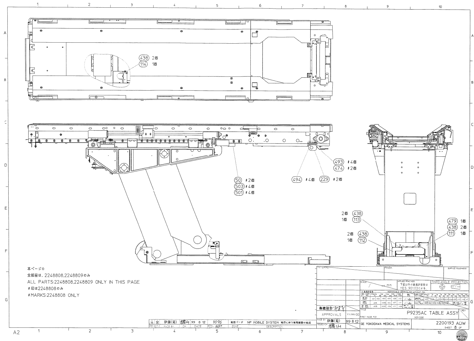
Figure 2-8 NP Lite Table (5194735ADW refer to 2200193ADW Sheet 8, Rev 15)
