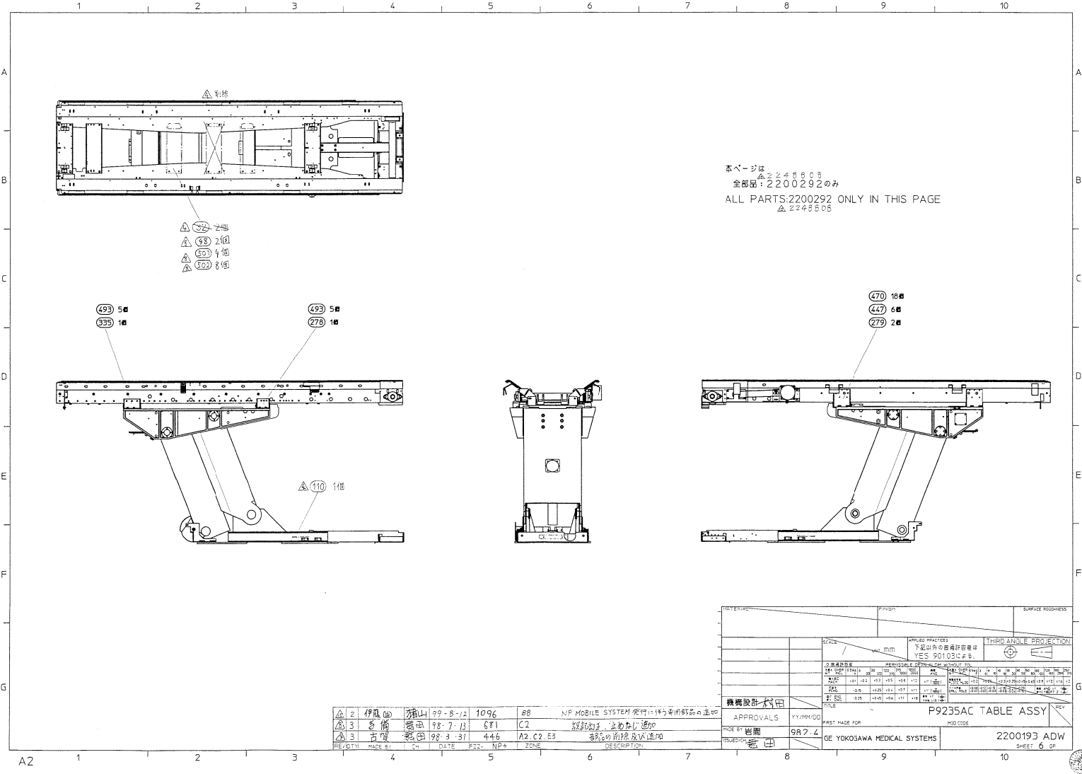
Figure 2-6 NP Lite Table (5194735ADW refer to 2200193ADW Sheet 6, Rev 15)
