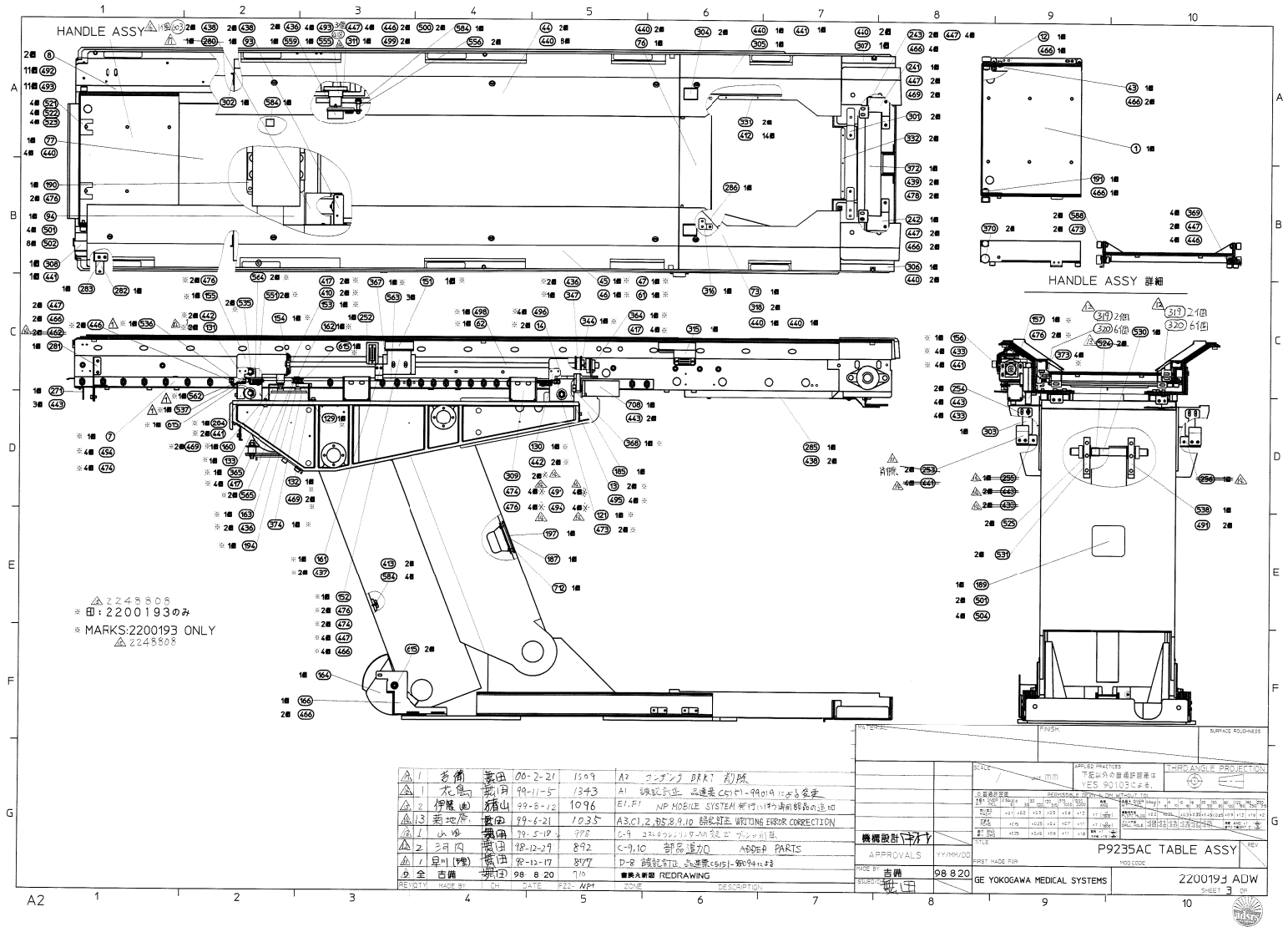
Figure 2-3 NP Lite Table (5194735ADW refer to 2200193ADW Sheet 3, Rev 17)
